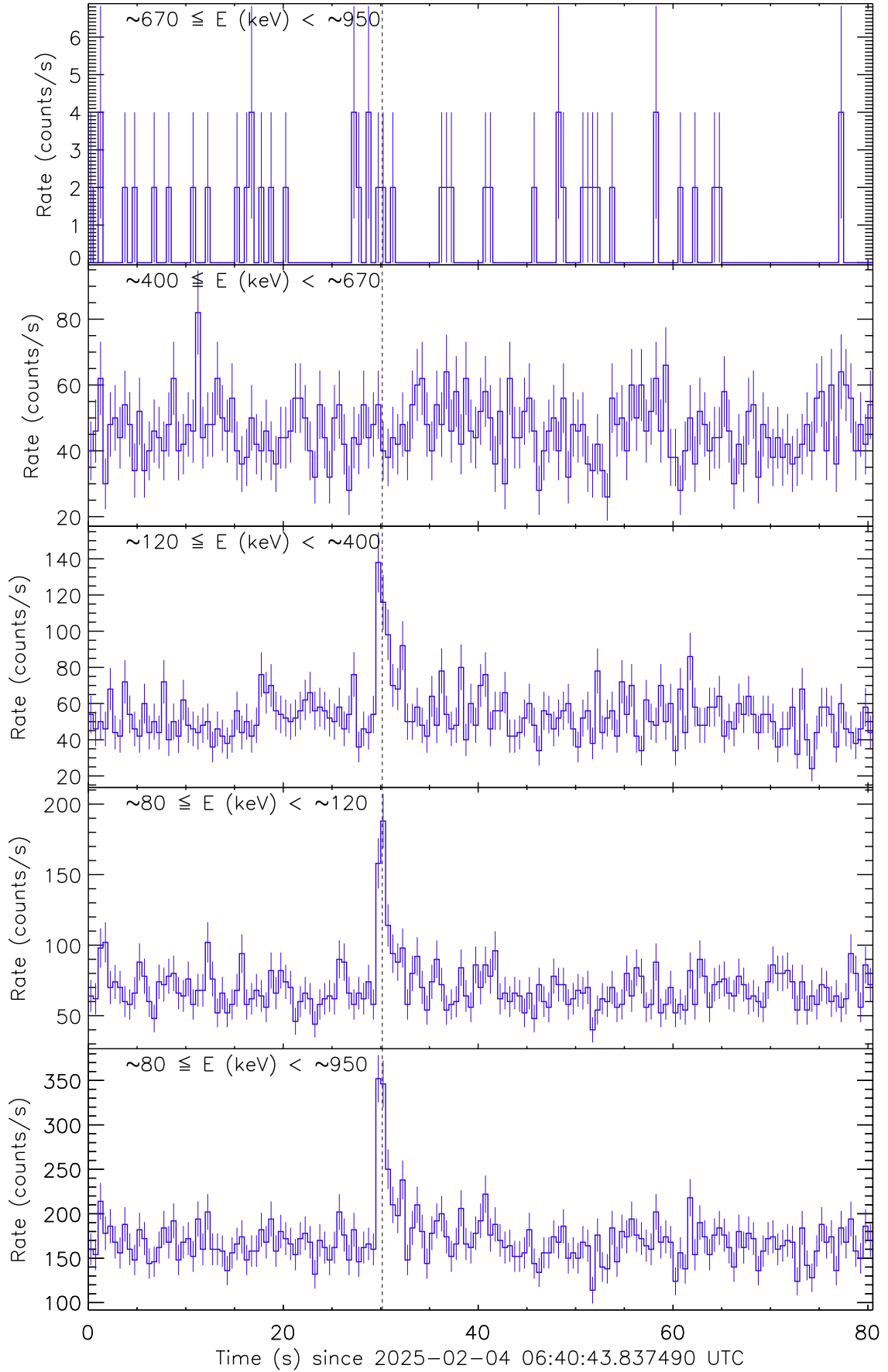
Figure 1: Raw count rate curve of GRB 250204B. The vertical dashed line marks the trigger time by Fermi/GBM.
