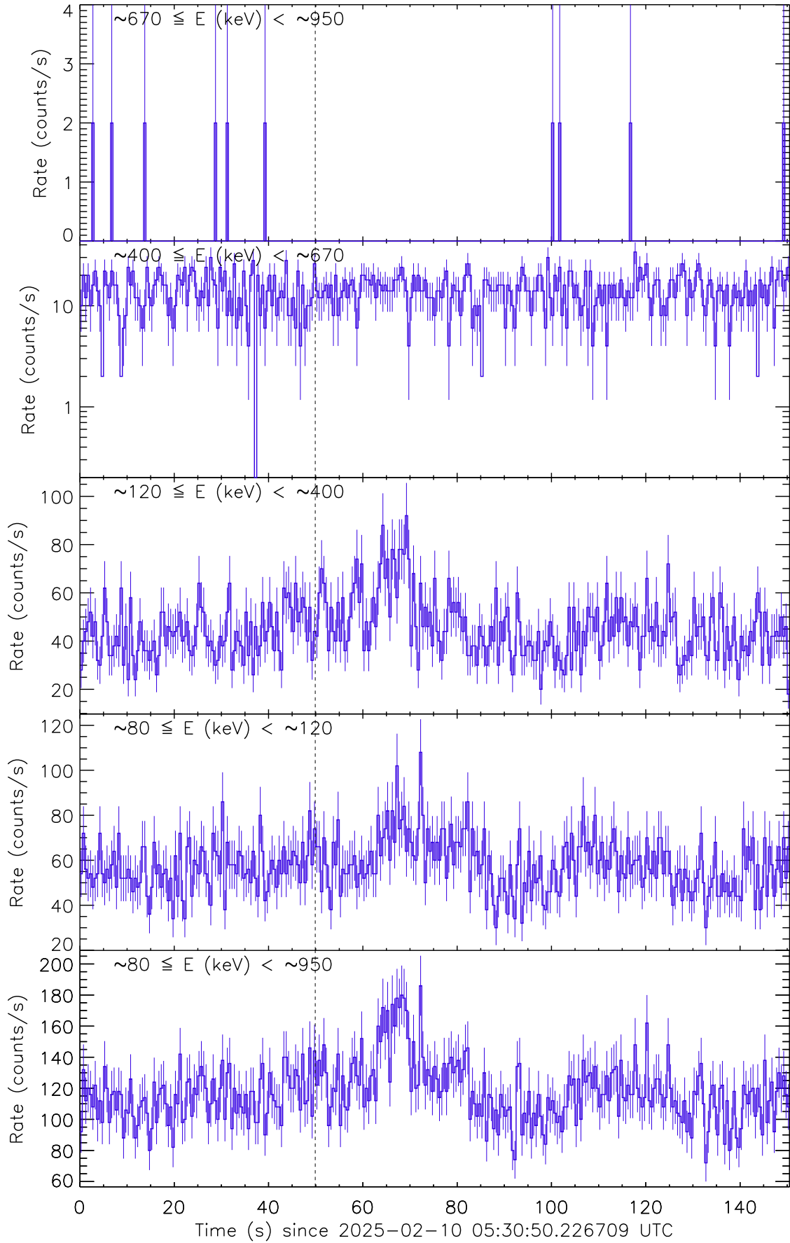
Figure 1: Raw count rate curve of GRB 250210A. The vertical dashed line marks the trigger time by Fermi/GBM.
