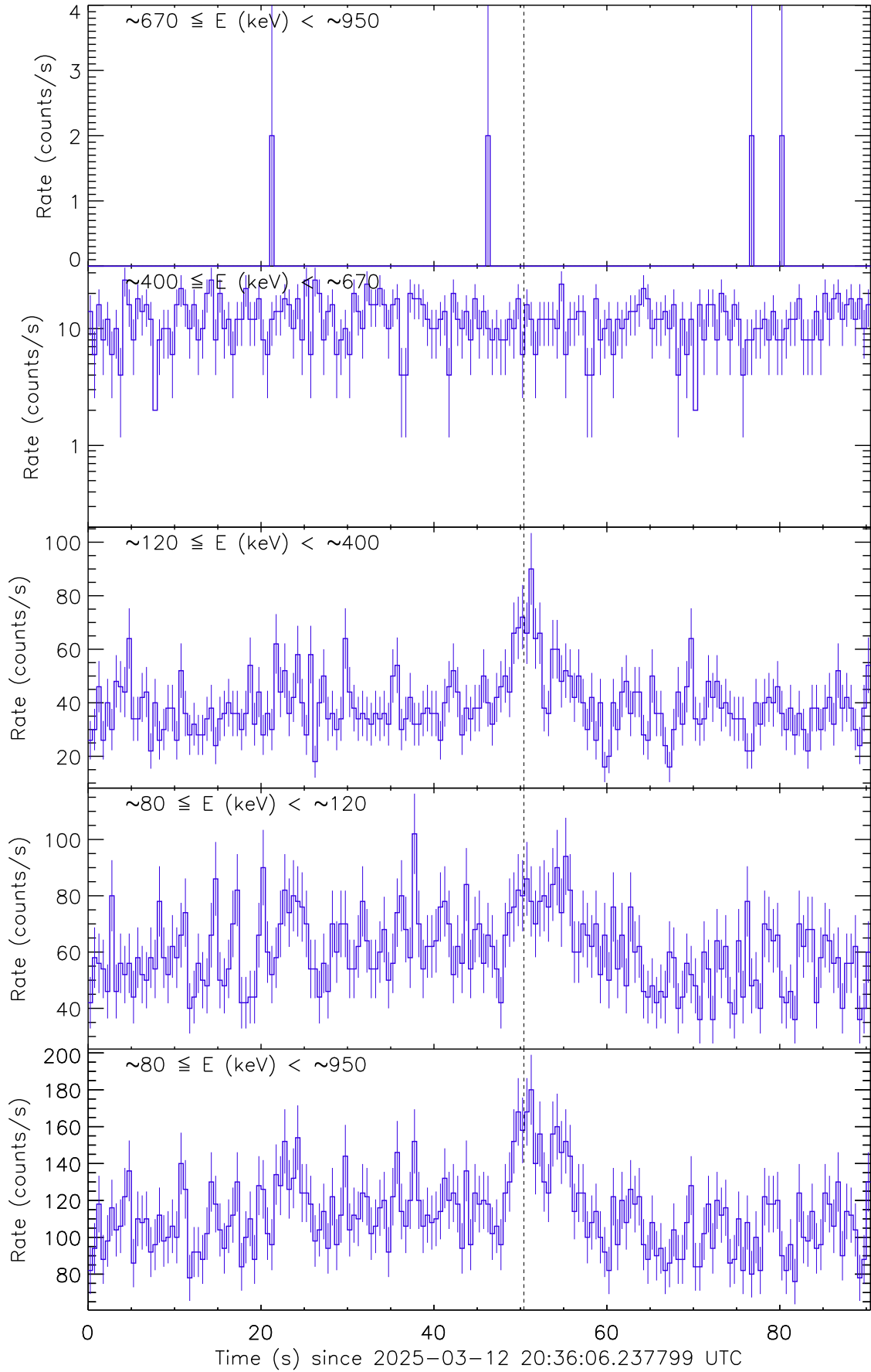
Figure 1: Raw count rate curve of GRB 250312B. The vertical dashed line marks the trigger time by Fermi/GBM.
