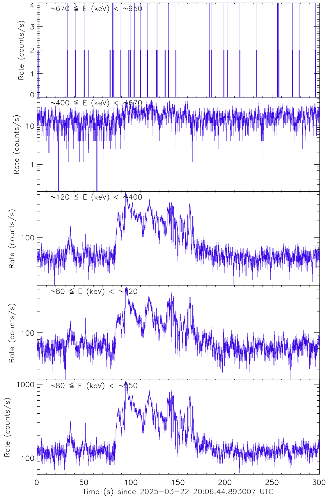
Figure 1: Raw count rate E curve of GRB 250322B. The vertical dashed line marks the trigger time by AstroSat/CZTI.
