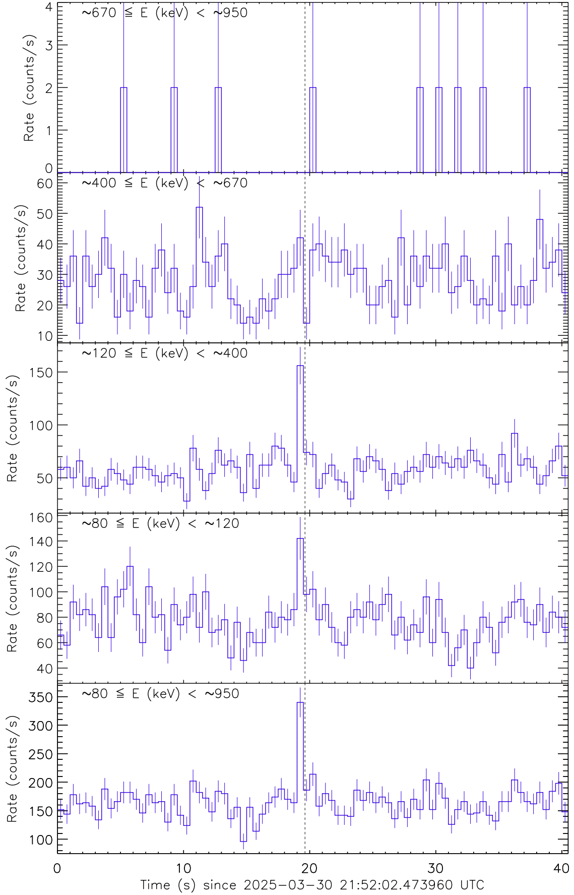
Figure 1: Raw count rate curve of GRB 250330B. The vertical dashed line marks the trigger time by Fermi/GBM.
