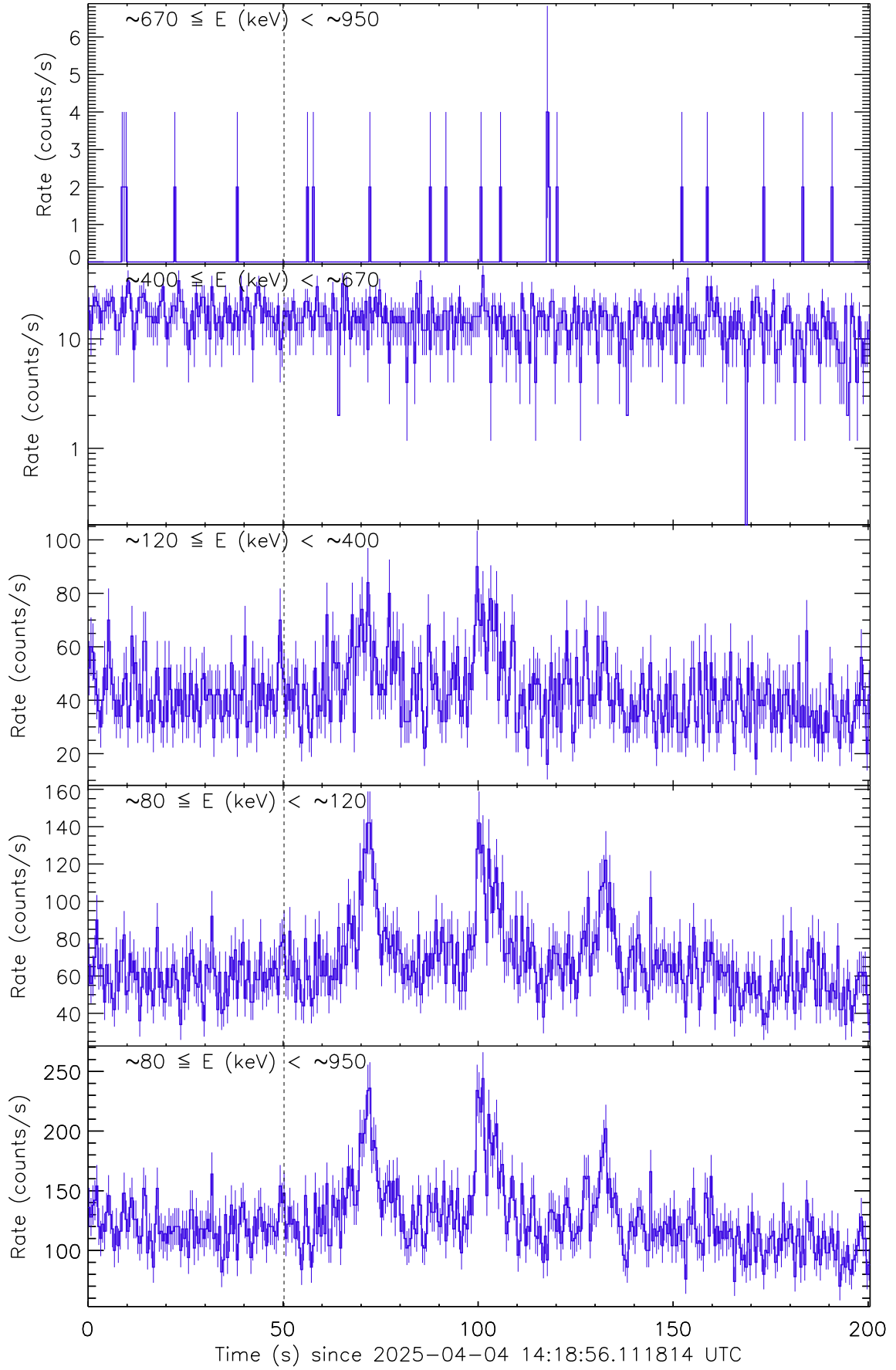
Figure 1: Raw count rate curve of GRB 250404A / EP250404a. The vertical dashed line marks the trigger time by Fermi/GBM.
