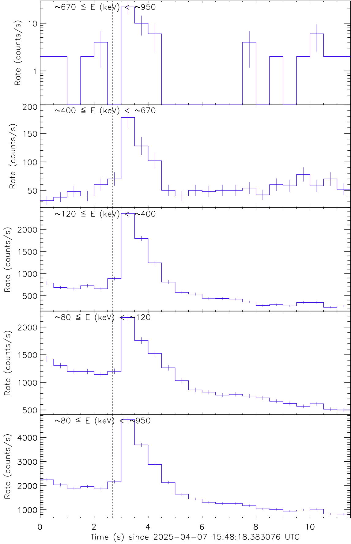
Figure 1: Raw count rate curve of GRB 250407A. The vertical dashed line marks the trigger time by Fermi/GBM.
