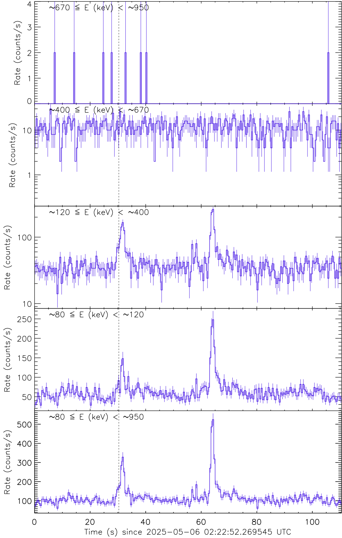
Figure 1: Raw count rate curve of GRB 250506A. The vertical dashed line marks the trigger time by Fermi/GBM.
