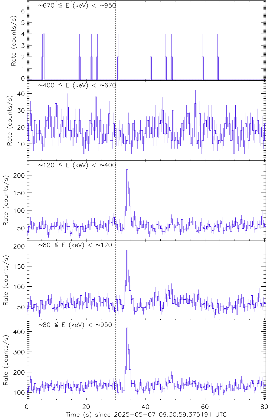
Figure 1: Raw count rate curve of GRB 250507B. The vertical dashed line marks the trigger time by Wind/Konus.
