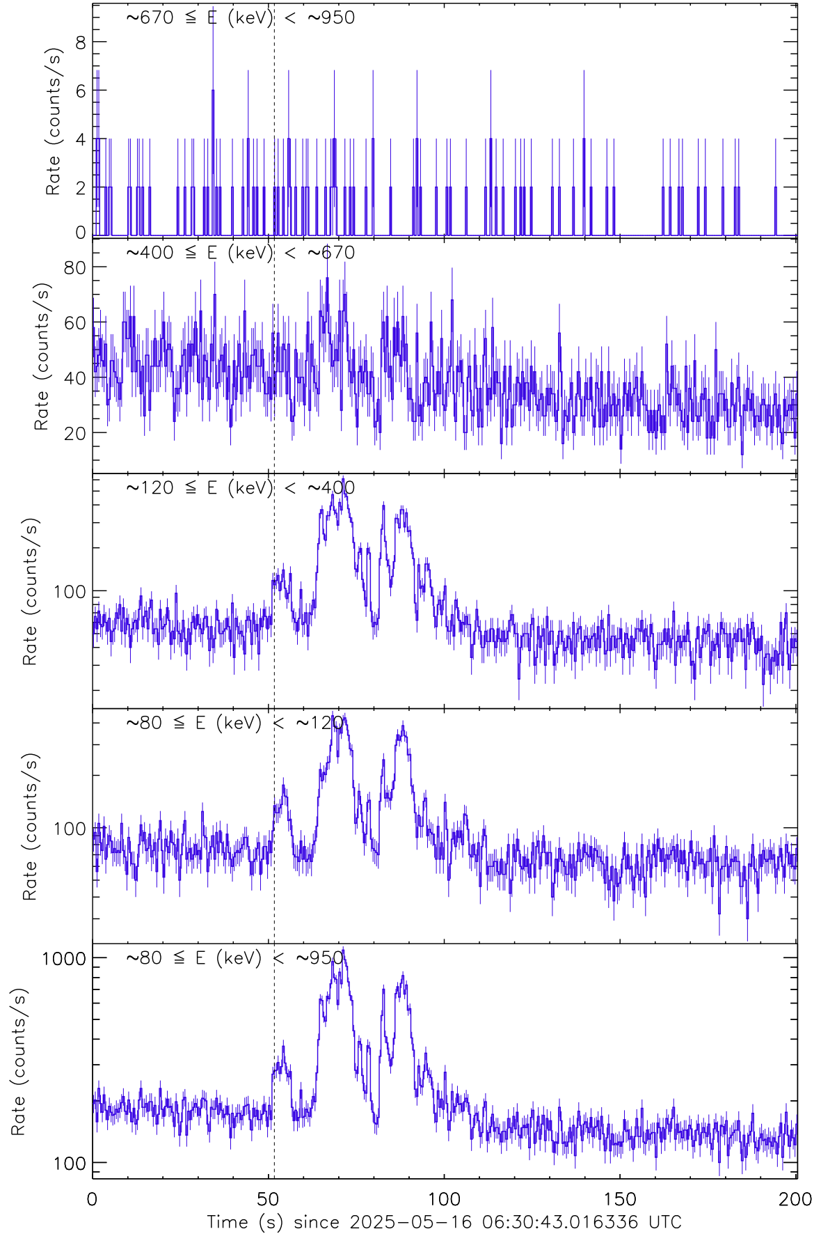
Figure 1: Raw count rate curve of GRB 250516B. The vertical dashed line marks the trigger time by GECAM-B.
