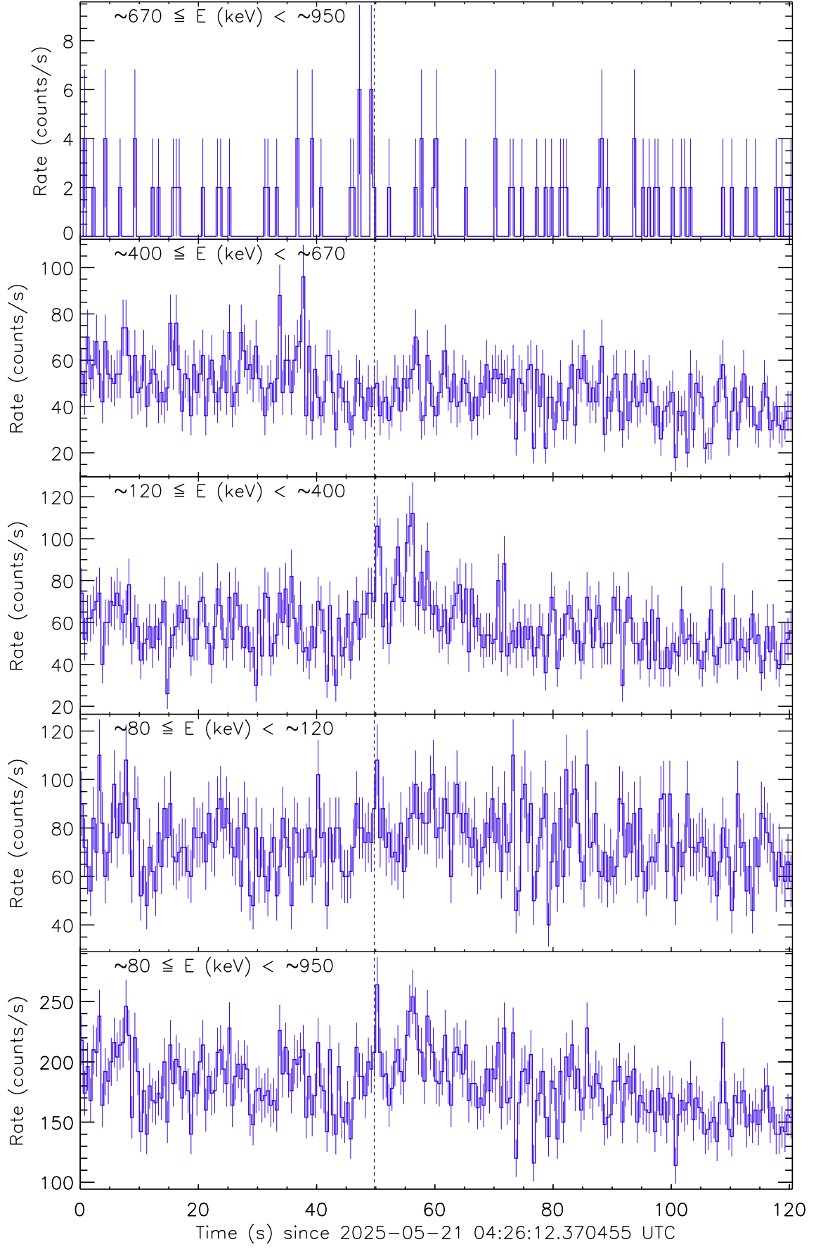
Figure 1: Raw count rate curve of GRB 250521A. The vertical dashed line marks the trigger time by Fermi/GBM.
