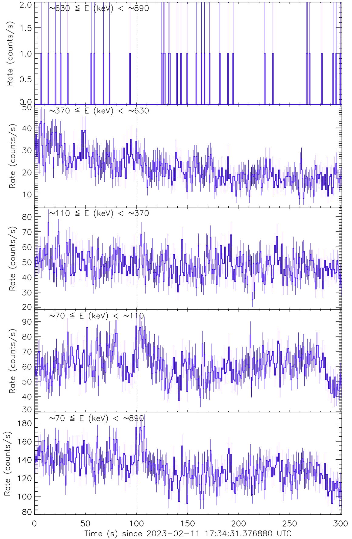
Figure 1: Raw count rate curve of LS V +44 17 / RX J0440.9+4431. The vertical dashed line marks the trigger time by Fermi/GBM.
